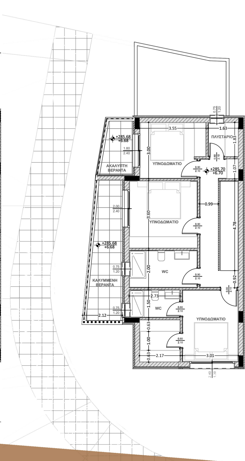
FIRST FLOOR
