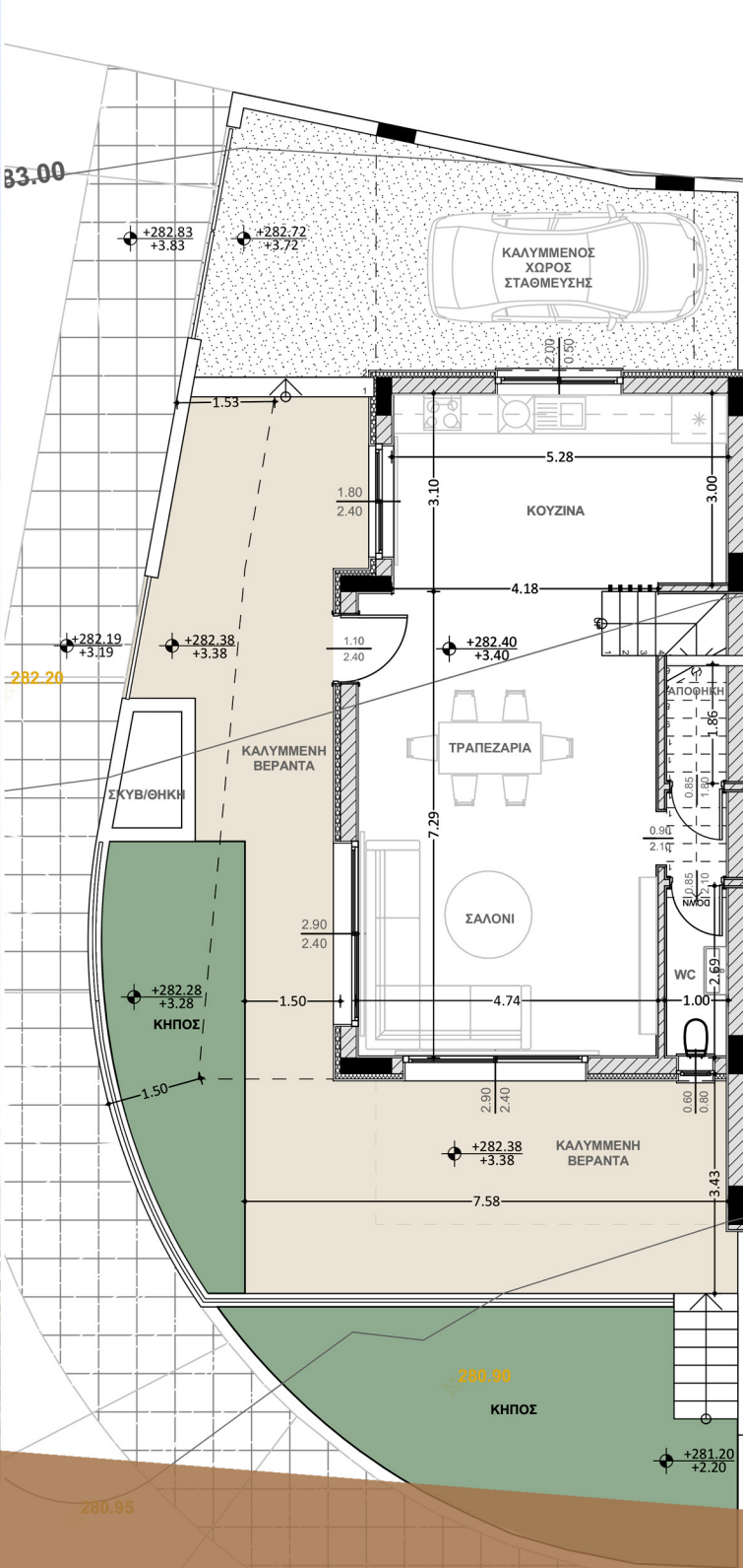
GROUND FLOOR
