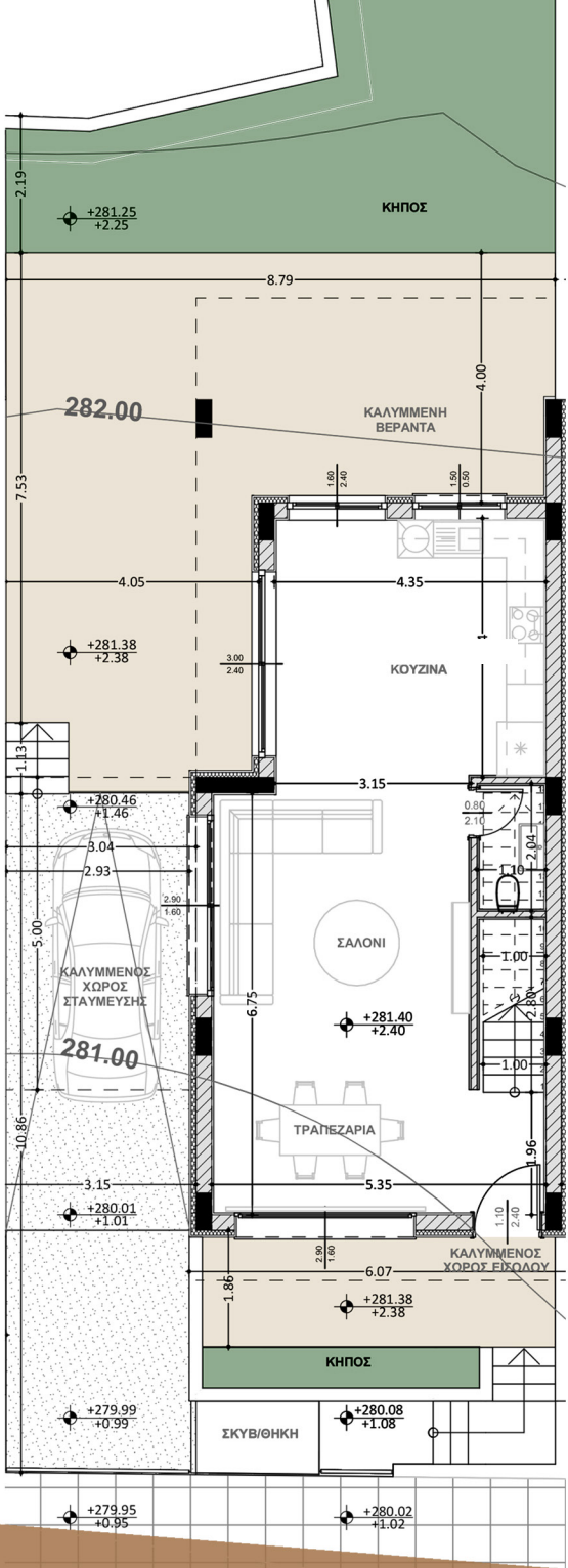
GROUND FLOOR
